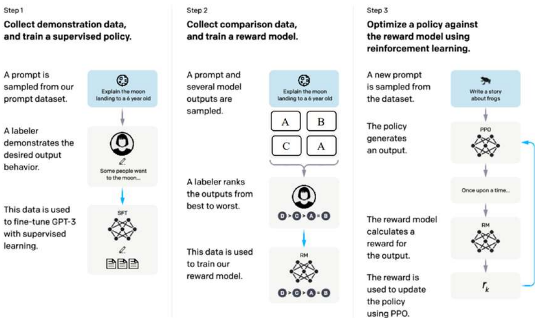
Figure 4-4. Taken from "training language models to follow instructions with human feedback" where A (explain gravity), B (explain war), or C (moon) is a natural satellite of D (people went to the moon)
