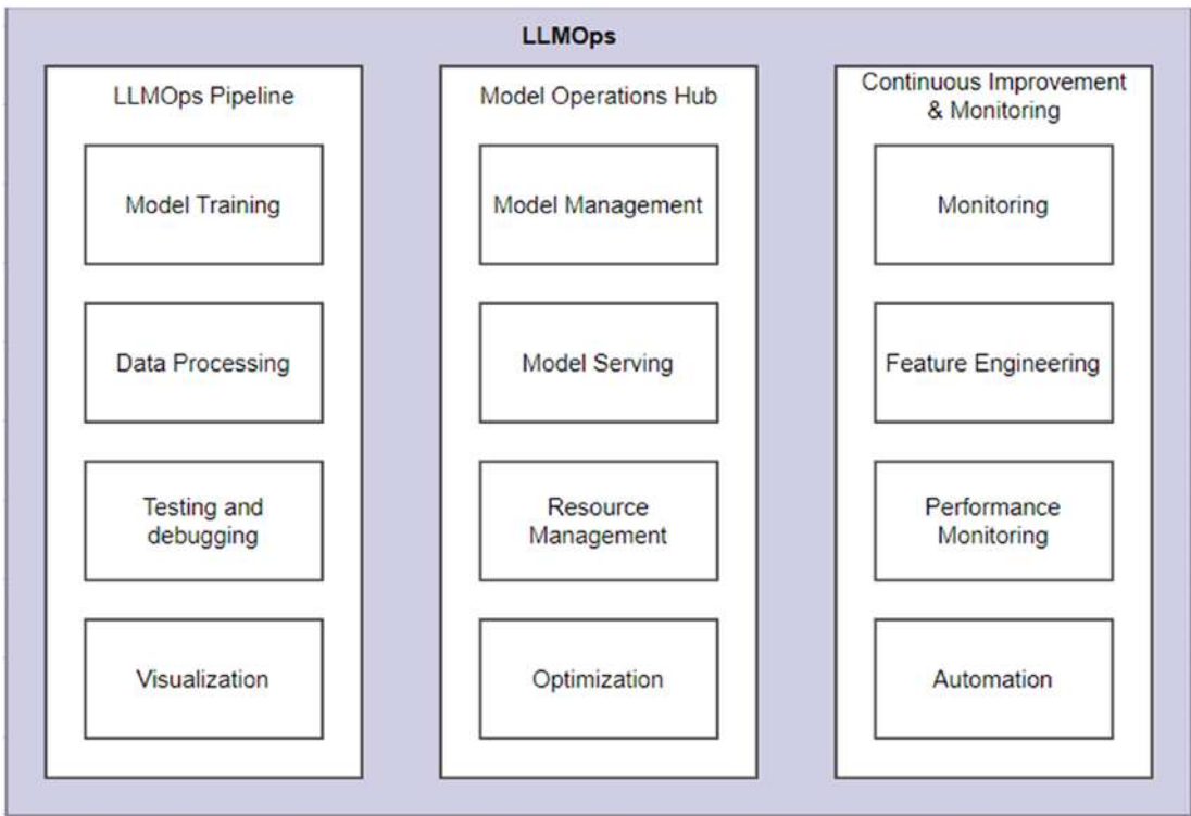
Figure 7-7. LLMOps
