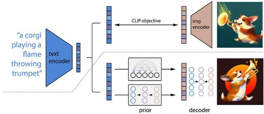
Figure 8-6. DALL-E 2
