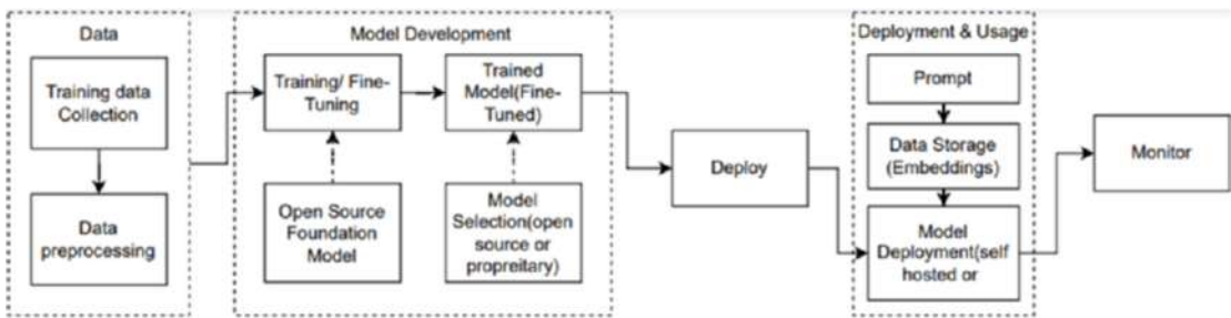
Figure 7-8. LLMOps workflow
