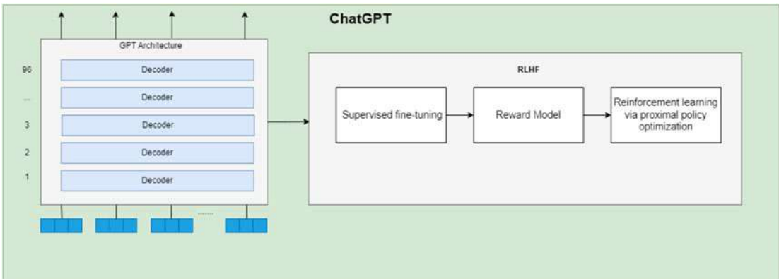
Figure 4-2. ChatGPT architecture
